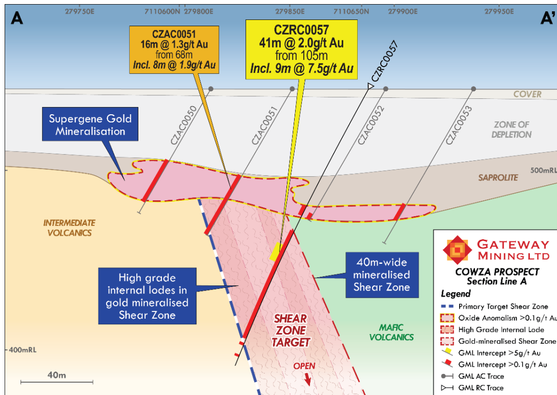
Figure 3: Cross section A-A' highlighting the new high-grade primary gold discovery at Cowza from RC hole CZRC057.
