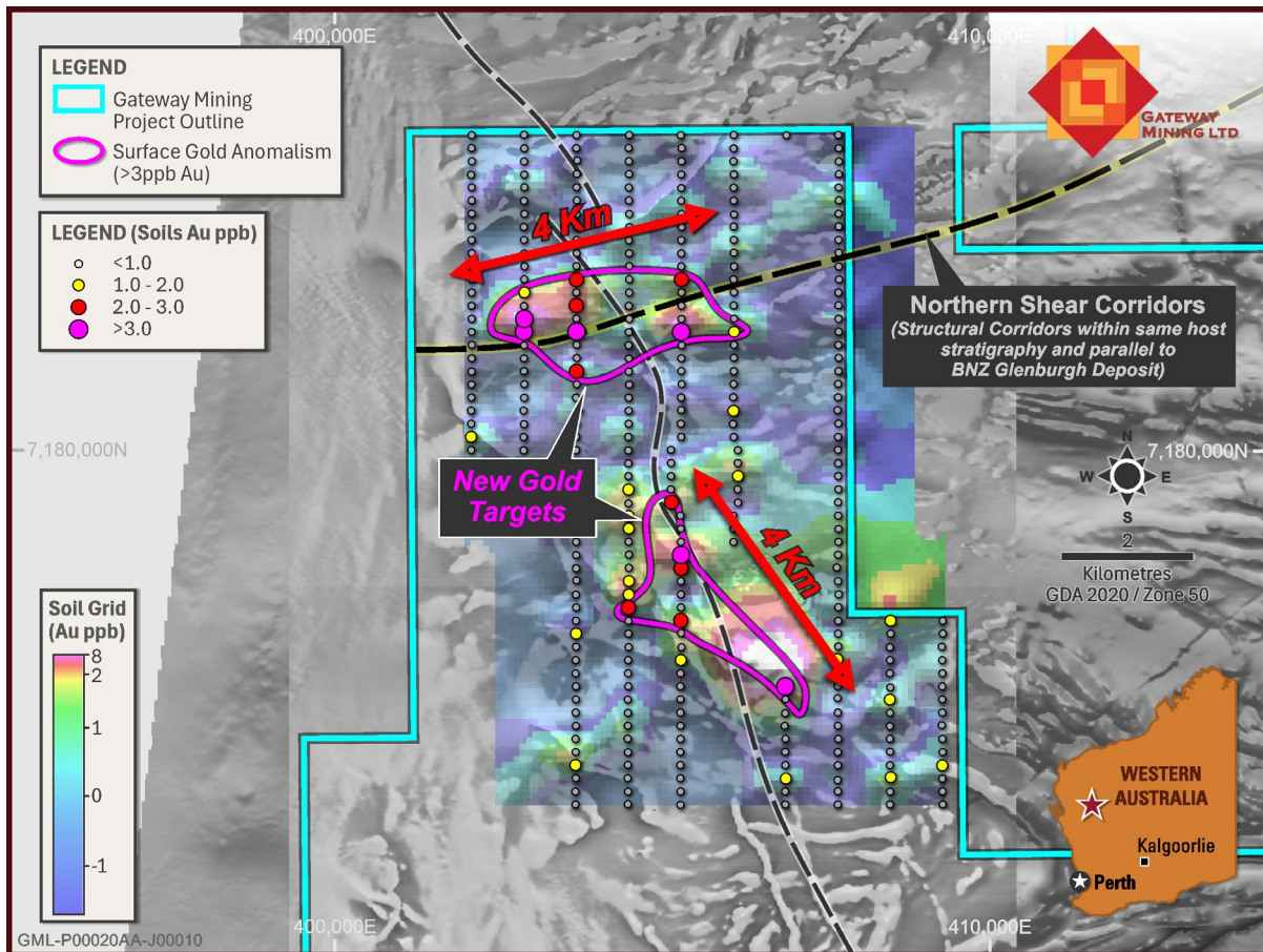
Figure 8: Peak gold in soil anomalism (ppb) in relation to key regional structures. Magnetic TMI image underlay.
