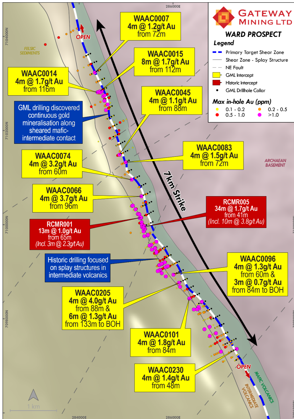
Figure 4: Plan view Ward Prospect. Recent GML AC results, focusing on the key mafic-intermediate contact, in relation to historic Ward drilling.
