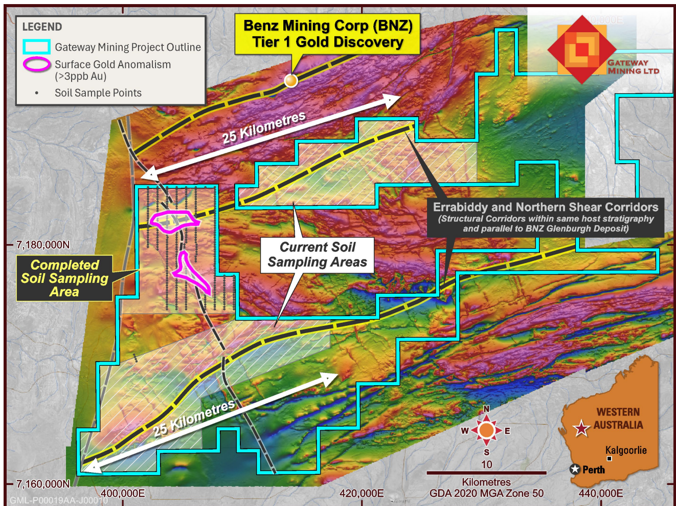
Figure 7: New coherent surface gold anomalies (pink outlines) in relation to regional structures and Benz Mining Corp (BNZ's) Glenburgh Gold Discovery. Magnetic TMI image underlay.
